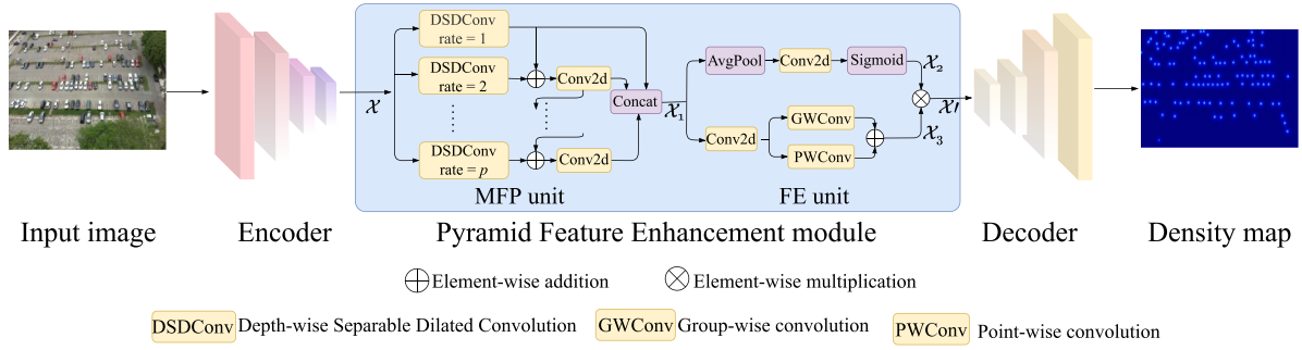
Figure 2. The pipeline of the PANet for vehicle counting.
