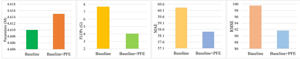
Figure 6. Ablation study on key modules of the PFE module.
