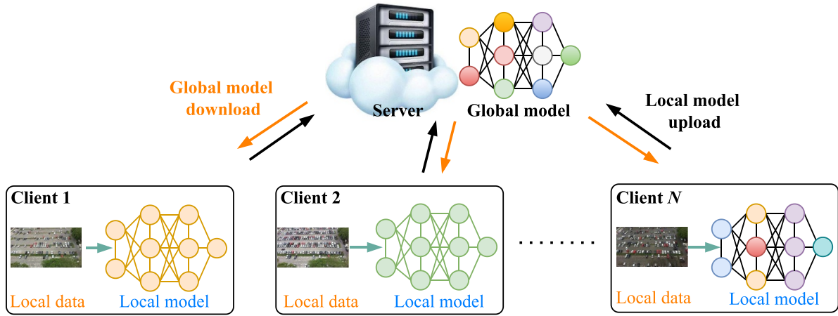
Figure 3. The overview of the federated learning framework.
