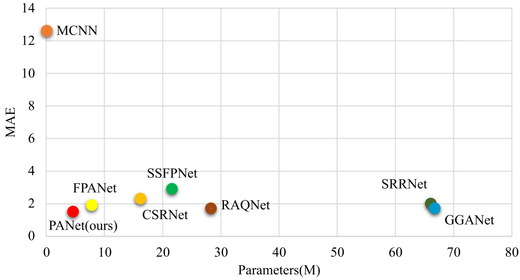
Figure 1. Comparison of the number of parameters and accuracy within the SOTA counting models on the PUCPR+ dataset. A lower mean absolute error (MAE) indicates a higher counting accuracy, and a larger number of parameters reflects a heavier network. These SOTA models include: MCNN [7], CSRNet [8], RAQNet [9], SRRNet [3], GGANet [10], FPANet [11], SSFPNet [12]. The proposed approach ensures high counting precision with a minimal number of parameters.
